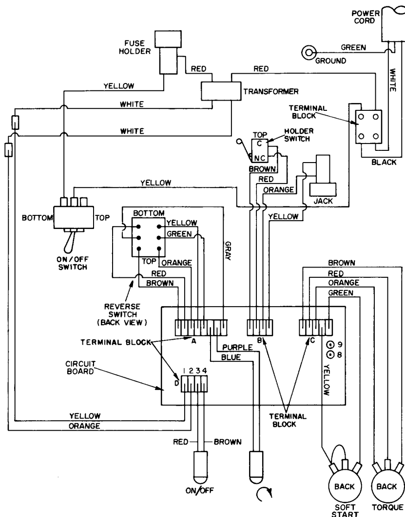
Wiring Diagram
